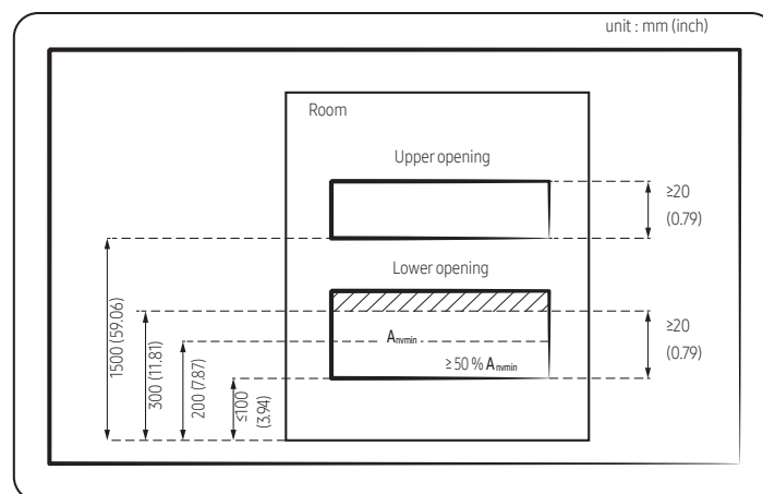
A min Minimal ventilation area
