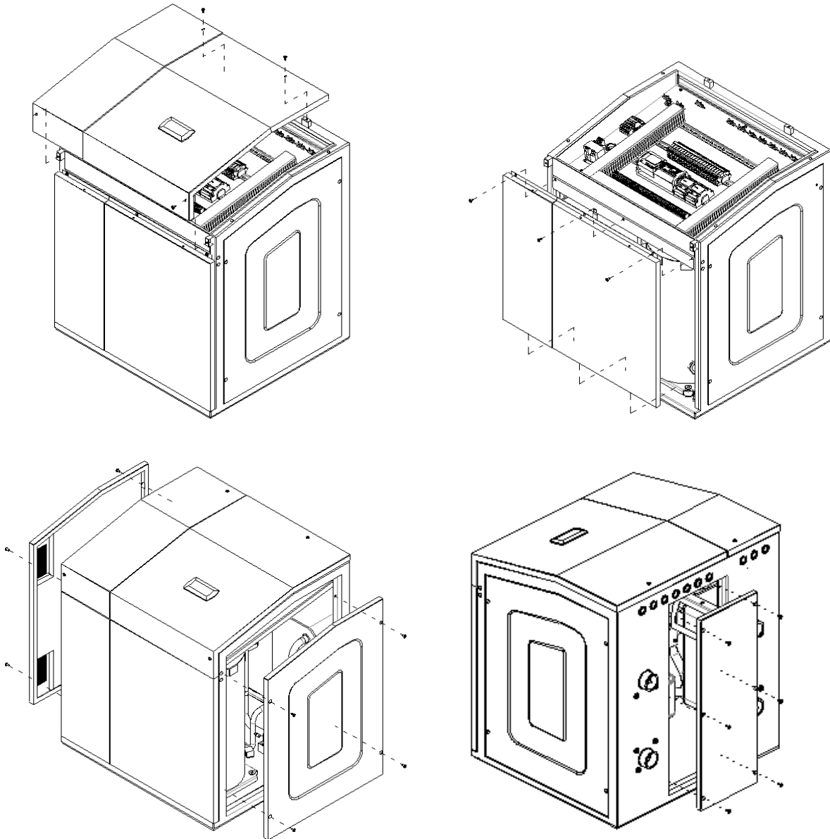
Figure 2.3. Disassembly of the covers of the VOLTA W-H models.
