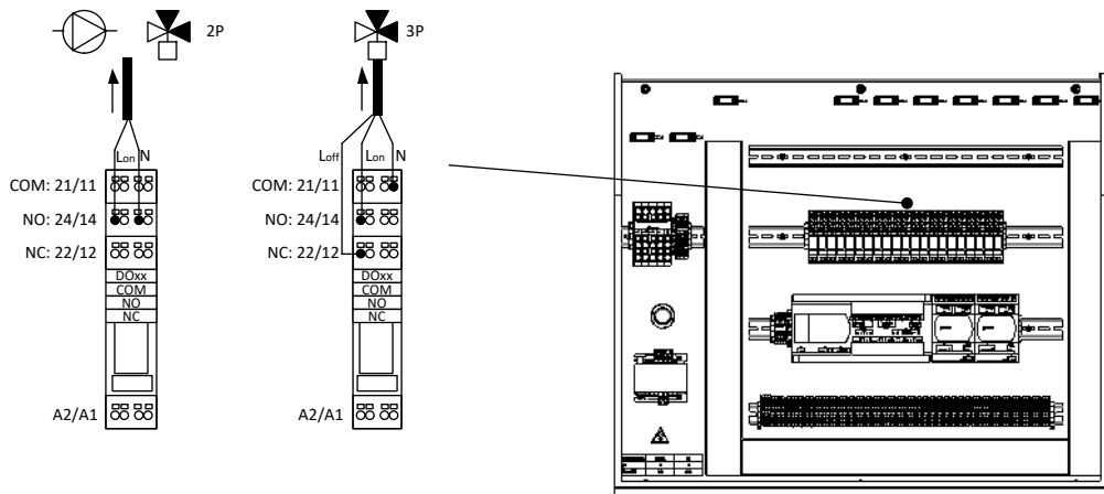
Figure 5.8. Example of digital output connections.
