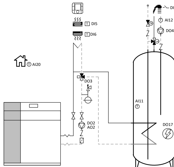
Figure 3.6. Wiring scheme of the DHW circuit
