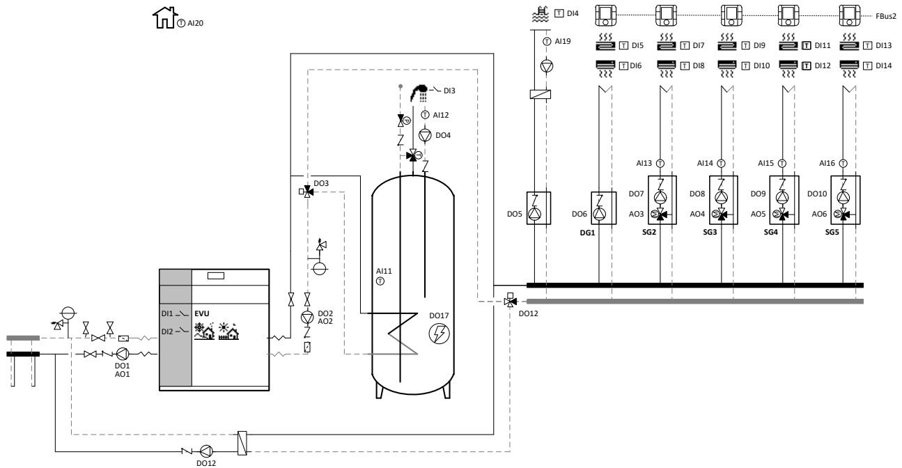
Figure 3.2. Wiring scheme directly to the heating / cooling system (VOLTA W-H-A models).
