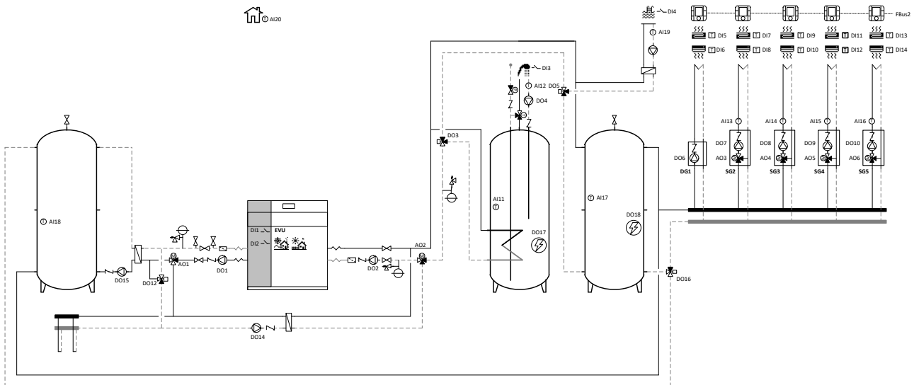
Figure 3.5. Wiring scheme using two buffer storage tanks with simultaneous production (VOLTA W-H-H models).
