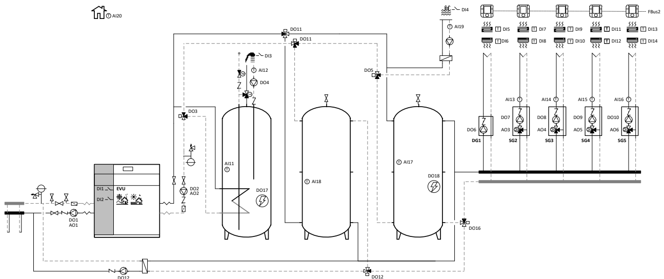
Figure 3.3. Wiring scheme using two buffer storage tanks (VOLTA W-H-A models).
