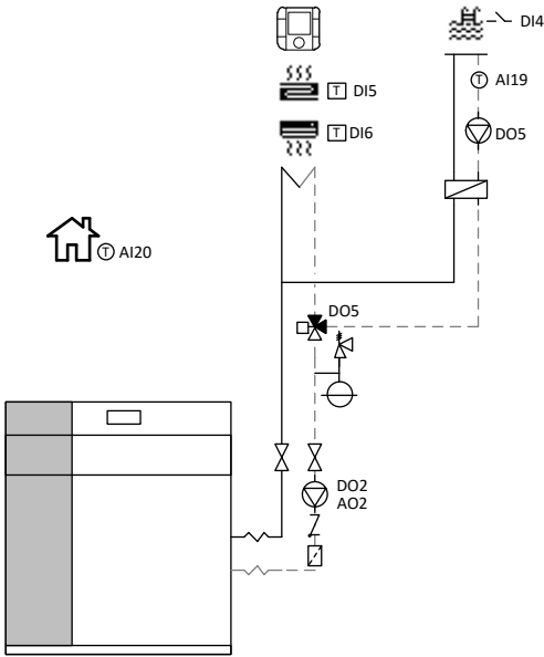
Figure 3.7. Pool production wiring schemes
