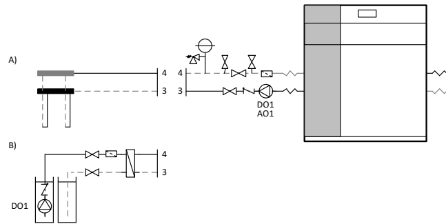
Figure 3.1. Brine circuit connection options.
