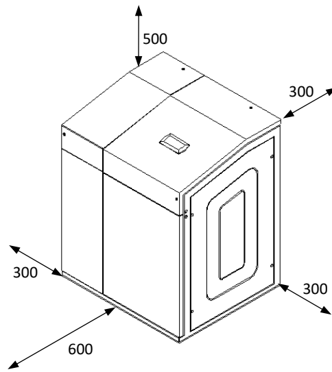
Figure 2.5. Minimum recommended service areas around the heat pump (amounts in mm).
