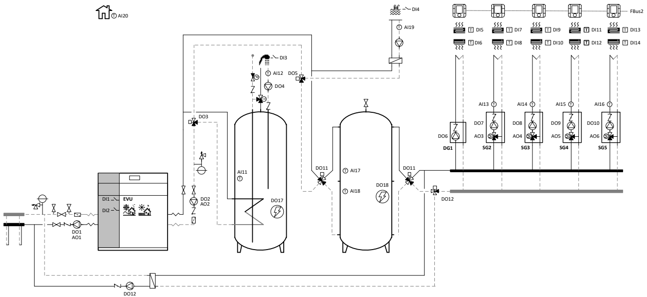
Figure 3.4. Wiring scheme using one buffer storage tanks (VOLTA W-H-A models).
